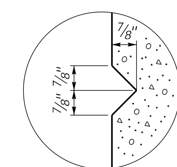
RUSTICATION GROOVE
